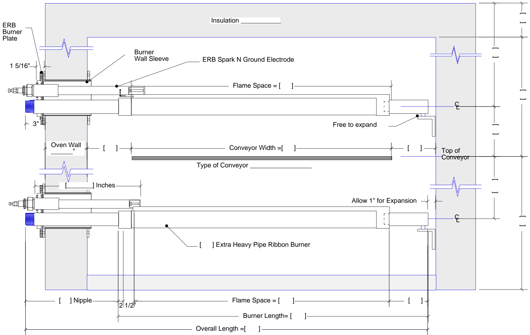
Tunnel Oven Cross sectional Drawing
