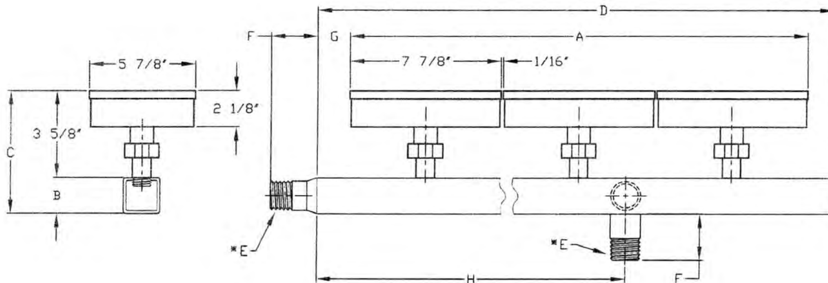
BURNER DIMENSIONS IN INCHES
