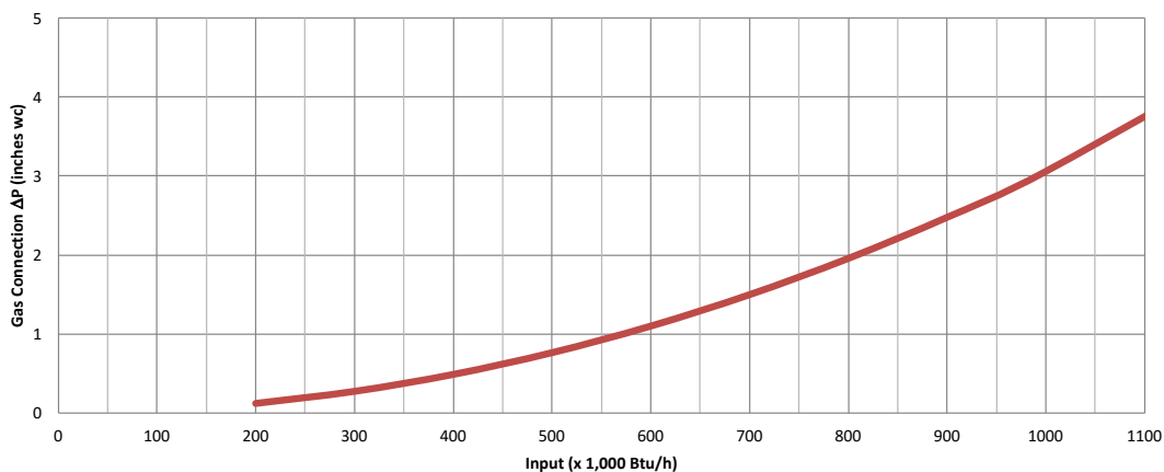
SuperFlame 1000 Natural Gas Pressure
