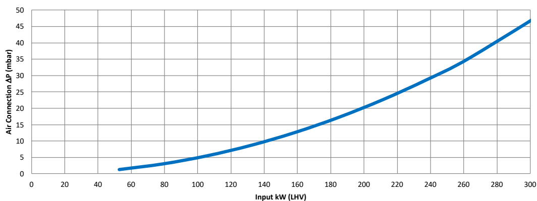
SuperFlame 1000 Air Pressure
