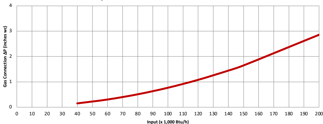
SuperFlame 150 Natural Gas Pressure
