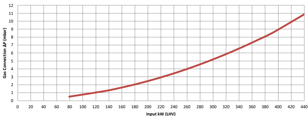
SuperFlame 1500 Natural Gas Pressure
