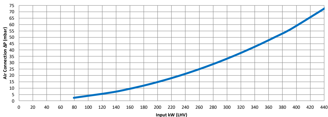
SuperFlame 1500 Air Pressure
