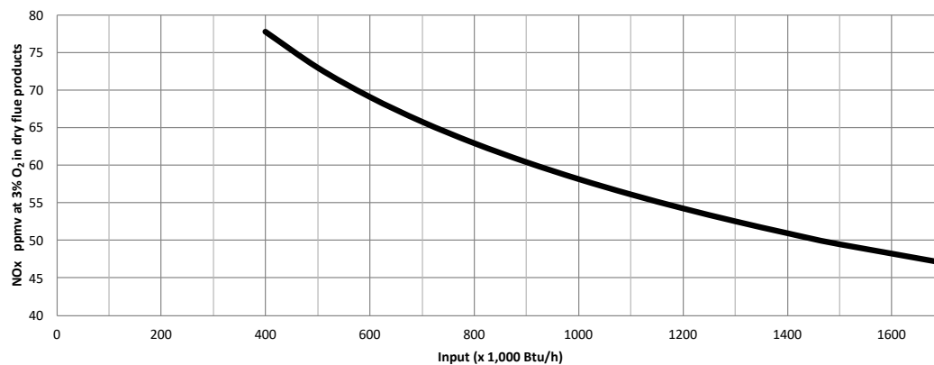
SuperFlame 1500 NOx Emissions
