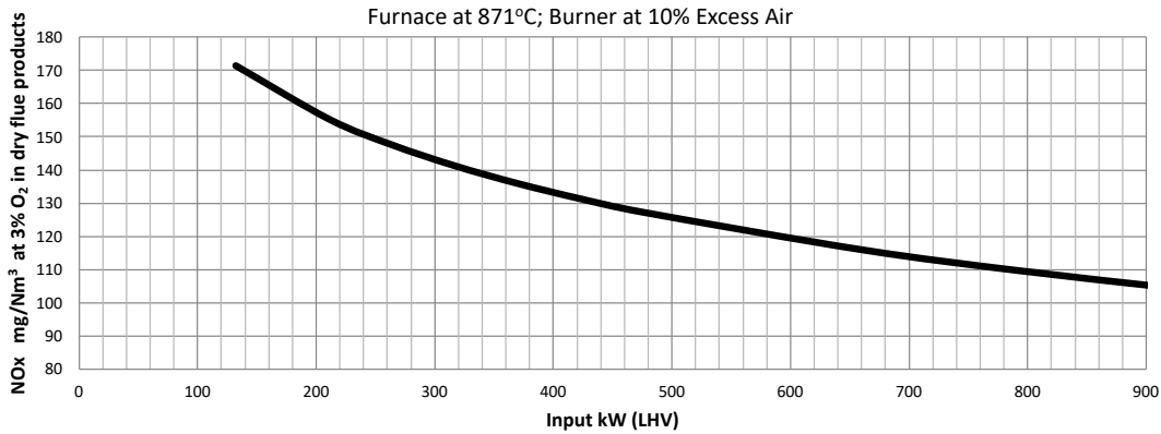
SuperFlame 3000 NOx Emissions
