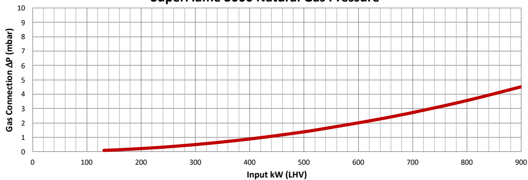
SuperFlame 3000 Natural Gas Pressure
