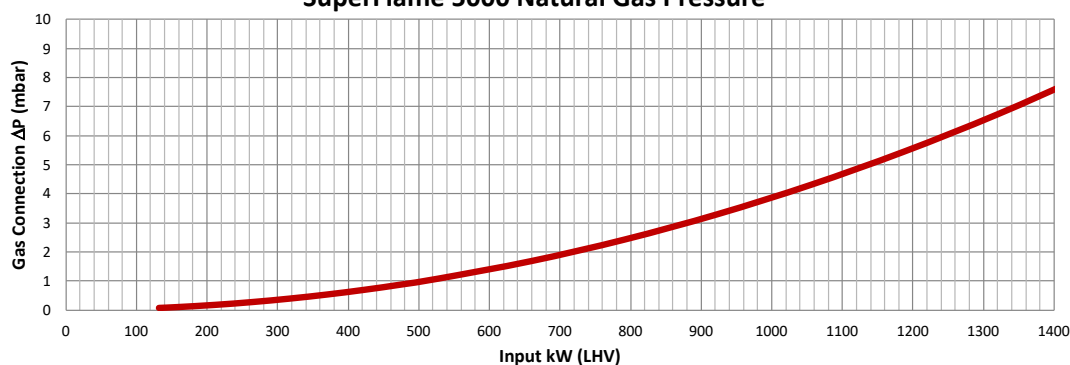
SuperFlame 5000 Natural Gas Pressure
