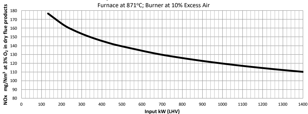
SuperFlame 5000 NOx Emissions
