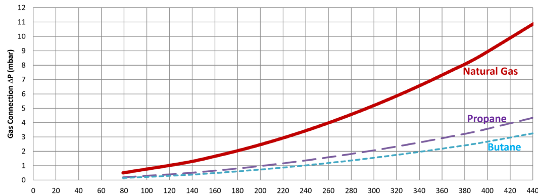
SuperFlame 1500 Fuel Gas Pressure
