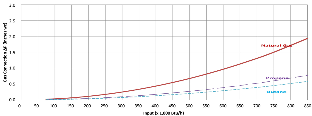
SuperFlame 750 Natural Gas Pressure
