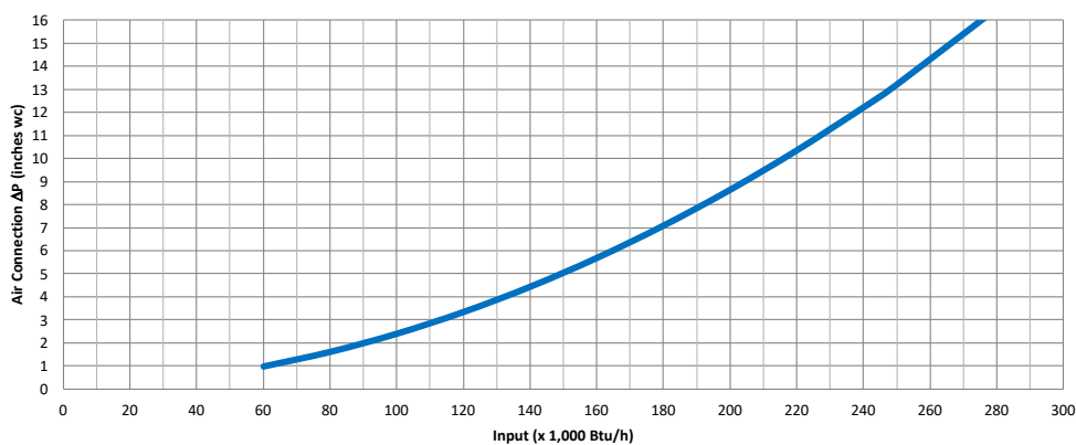
SuperFlame 250 Air Pressure
