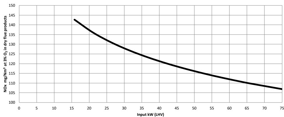
SuperFlame 250 NOx Emissions
