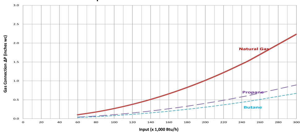
SuperFlame 250 Natural Gas Pressure
